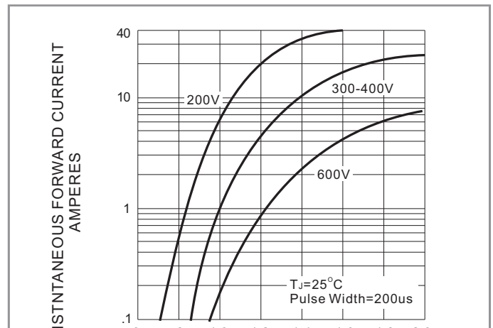
Fig.4- TYPICAL INSTANTANEOUS FORWARD CHARACTERISTIC
