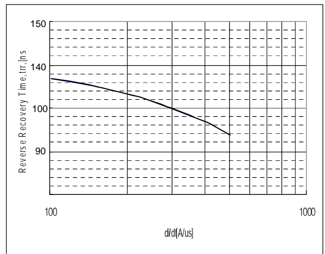
Fig. 2 : Typical Reverse Recovery Time vs. -di/dt
