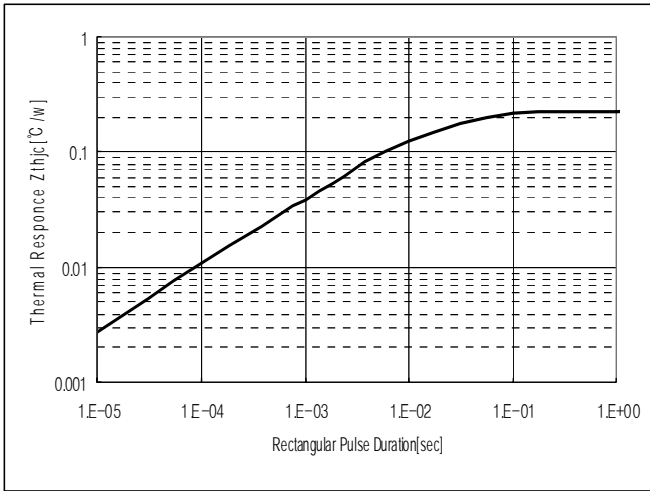
Fig. 3 : Transient Thermal Impedance( Z_{thjc} ) Characteristics
